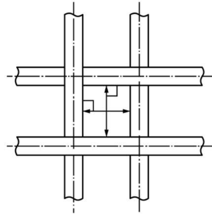
FIG. A1.4 Configuration of Twilled Weaves
