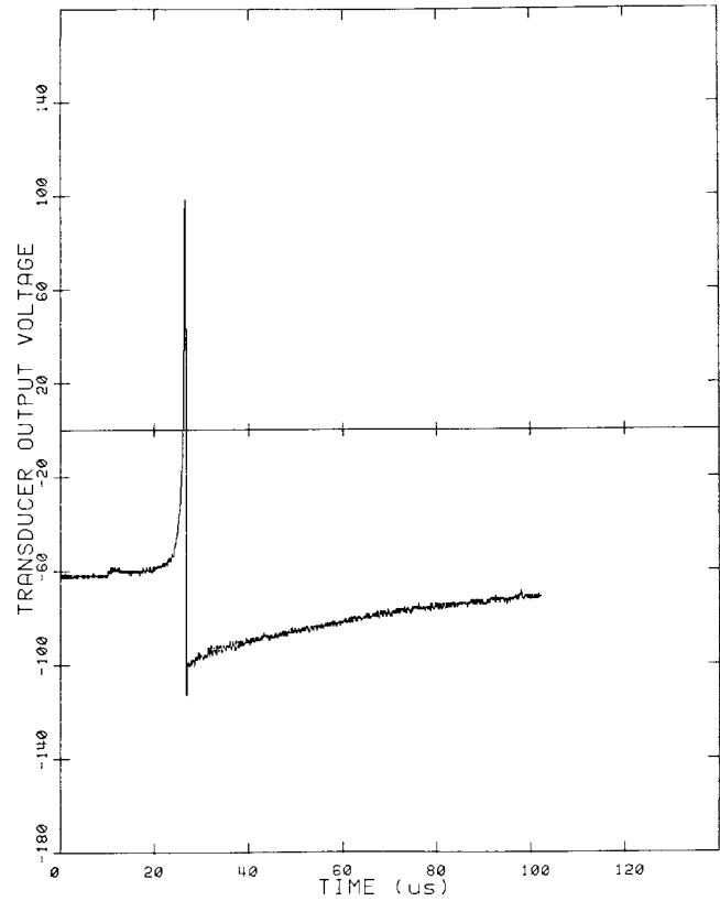
FIG. 9 A Typical Calibration—Voltage Versus Time Waveform from the Standard Transducer as Captured by the Transient Recorder
