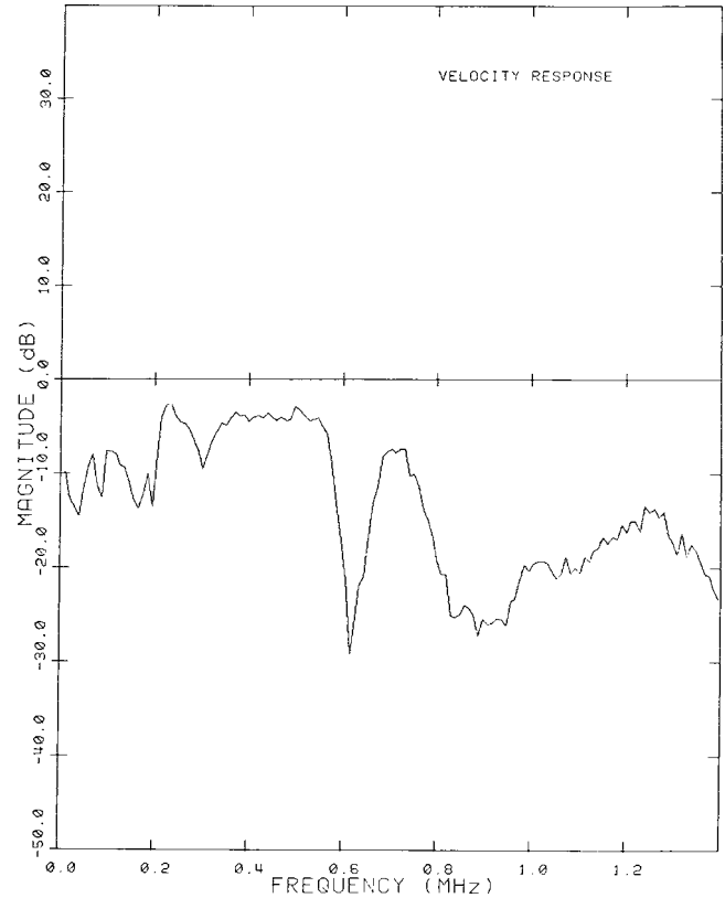
FIG. 15 Magnitude Response of the Unknown Transducer as Obtained by Division of the Ordinates of Fig. 13 by Those of Fig. 11
