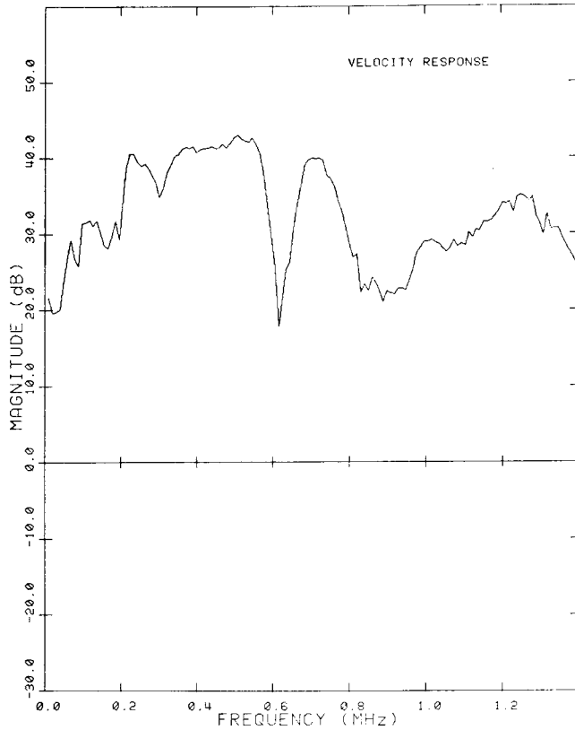
FIG. 13 Spectrum Magnitude as Obtained by Performing a Fast Fourier Transform on the Data of Fig. 10
