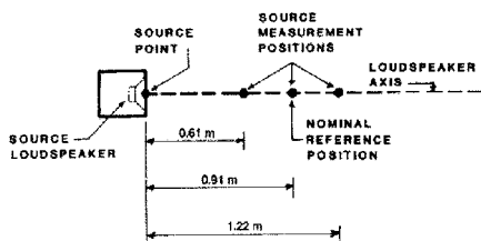
FIG. 5 Measurement Positions for Reference Levels, (Plan View)
