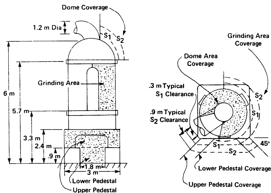
FIG. 3 Side View and Top View of Pulverizer
