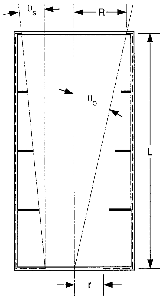
FIG. A1.1 Collimator Design
