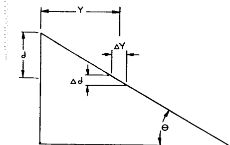
FIG. 1 Cross Section of Angle-Lapped Specimen
