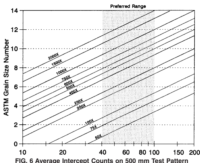
Fig. 6 shows the relationship between the average intercept count and the microscopically determined ASTM grain size number as a function of magnification.
