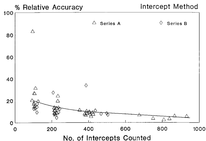
FIG. X1.4 Relationship Between the Number of Intercepts or Intersections Counted and the Percent Relative Accuracy for the Intercept Method
