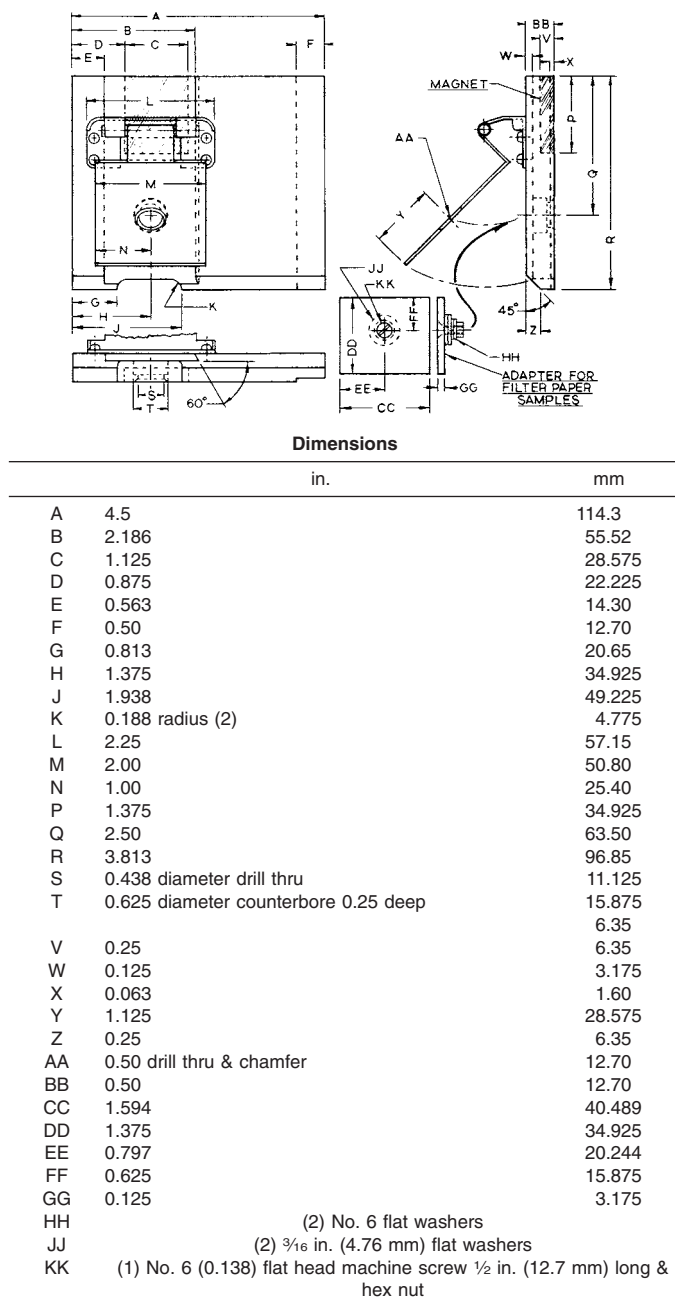
FIG. 2 Sample Holder for the Turner Fluorometer
