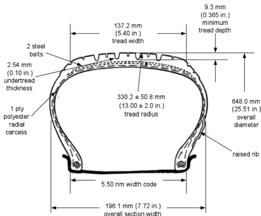
FIG. 3 Tire Cross Section
