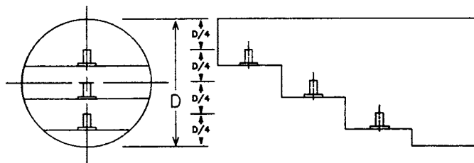
FIG. 1 Typical Distance-Amplitude Reference Block Configuration for the Ultrasonic Testing of Large Metal and Metal Alloy Bars of from 1 to 10 in. (25.4 to 254.0 mm) Diameter and Larger
