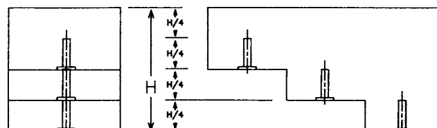
FIG. 3 Typical Distance-Amplitude Reference Block for the Ultrasonic Testing of Large Square or Rectangular Bars Greater than 1 in. (25.4 mm)
