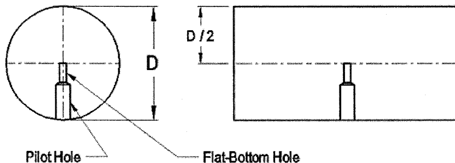
FIG. A1.1 Flat-Bottom Hole Placed at the Center of a Round Bar by This Method
