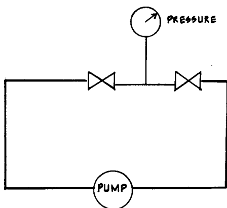
FIG. 4 Pressure Gauge
