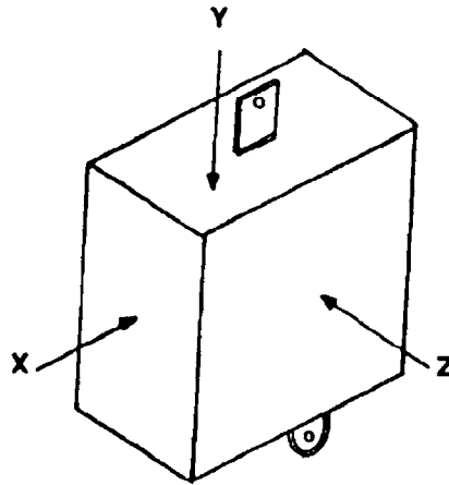
FIG. 6 Orientation of Noncylindrical Semiconductor Device to Direction of Accelerating Force
