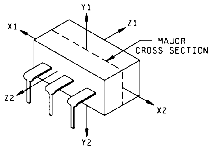
FIG. 3 Dual In-Line Package
