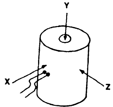
FIG. 7 Orientation of Cylindrical Semiconductor Device to Direction of Accelerating Force
