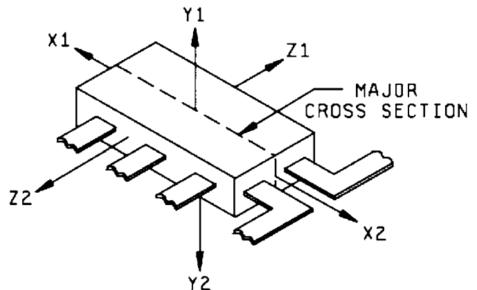
FIG. 2 Radial Lead Flat Packages
