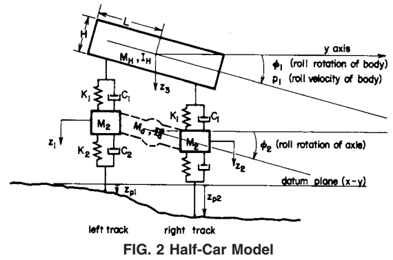
FIG. 2 Half-Car Model
