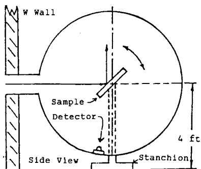
FIG. 2 Integrating Sphere (Reflectance Mode)
