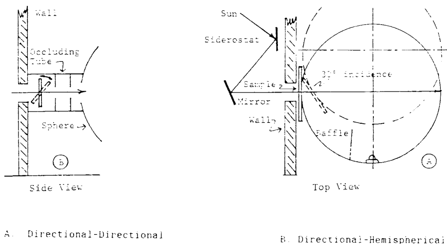
FIG. 1 Integrating Sphere (Transmittance Modes)
