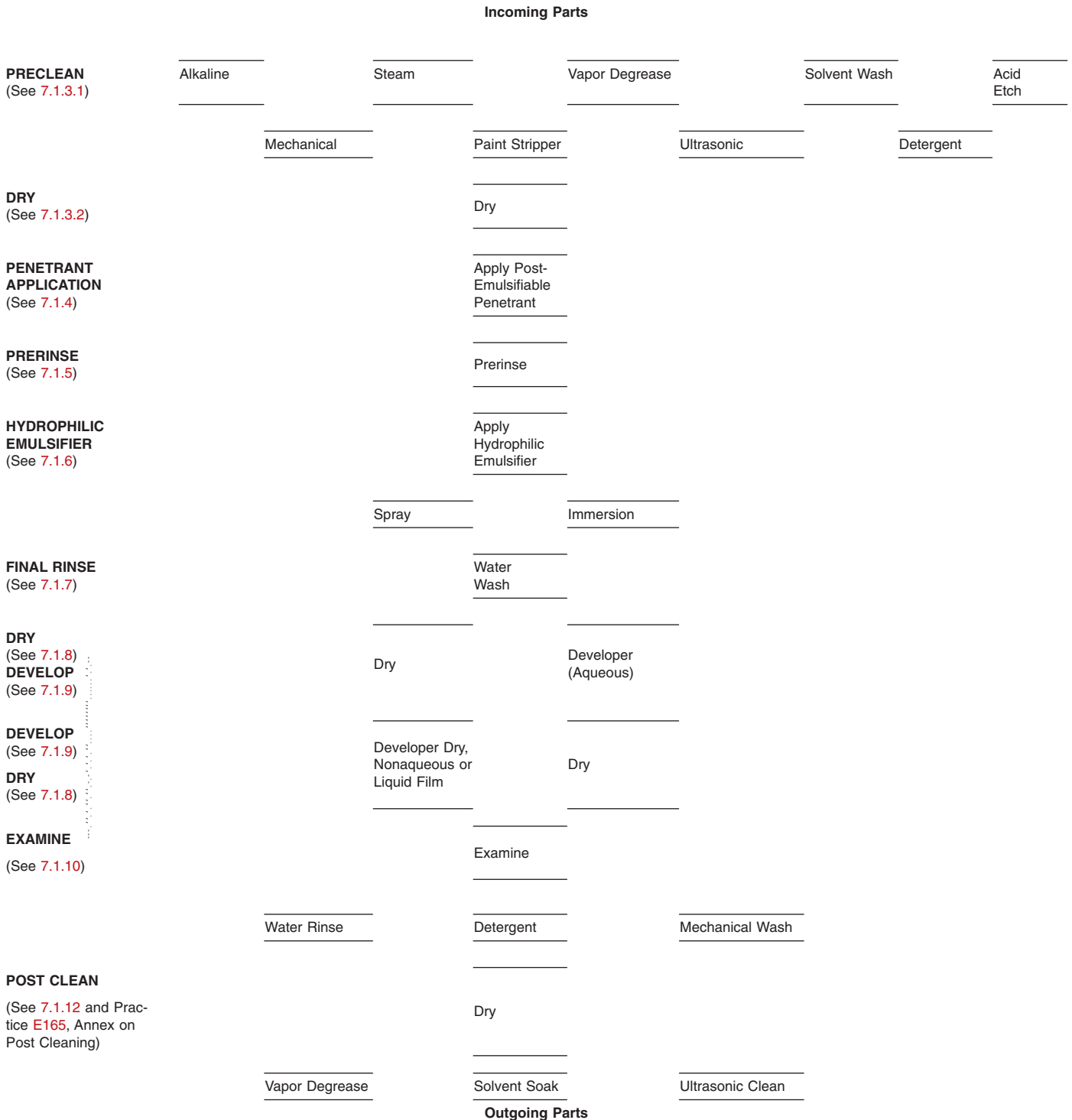
FIG. 1 General Procedure Flowsheet for Fluorescent Penetrant Examination Using the Water-Washable Process
