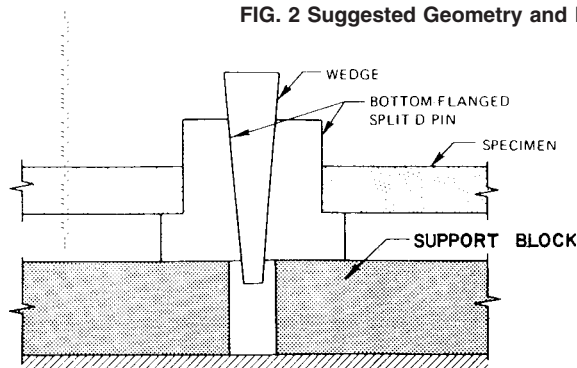
FIG. 3 Sectional View of a Loading Arrangement That May Be Helpful When Testing Specimens at Higher Temperatures
