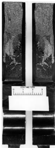
FIG. A1.4 Fracture Surface of a CCA Specimen Showing a Large Remaining Ligament Aligned with the Direction of Crack Propagation
