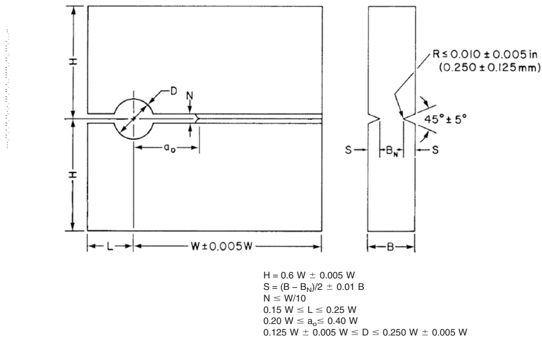
FIG. 5 Geometry and Dimensions of a Crack-Line-Wedge-Loaded Compact-Crack-Arrest (CCA) Test Specimen that is Satisfactory for Low and Medium Strength Steels
