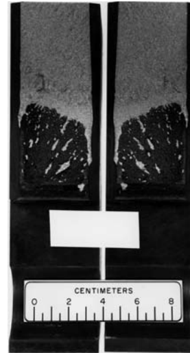
FIG. A1.10 Fracture Surface of a CCA Specimen with a Tunneled but Acceptable Crack Front
