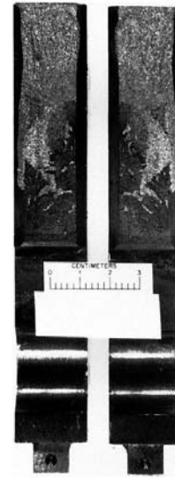
FIG. A1.4 Fracture Surface of a CCA Specimen Showing a Large Remaining Ligament Aligned with the Direction of Crack Propagation
