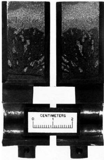
FIG. A1.6 Fracture Surface of a CCA Specimen Showing a Moderate Degree of Ligamentation
