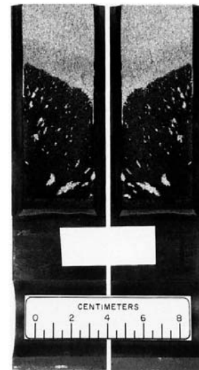
FIG. A1.9 Fracture Surface of a CCA Specimen with a Slanted and Nearly Straight Crack Front
