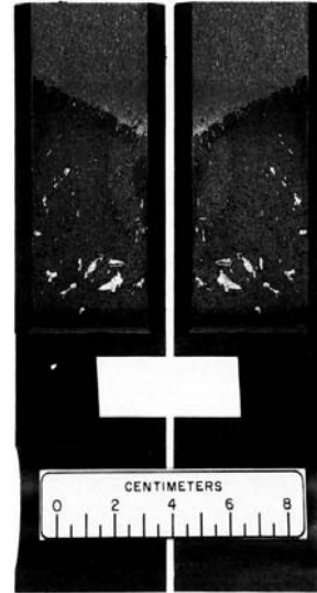
FIG. A1.8 Fracture Surface of a CCA Specimen with a Slanted and Straight Crack Front
