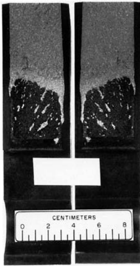
FIG. A1.10 Fracture Surface of a CCA Specimen with a Tunneled but Acceptable Crack Front
