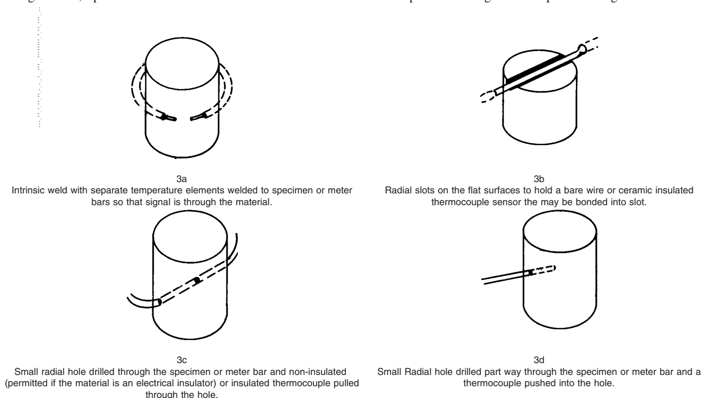
FIG. 3 Thermocouple Attachments
