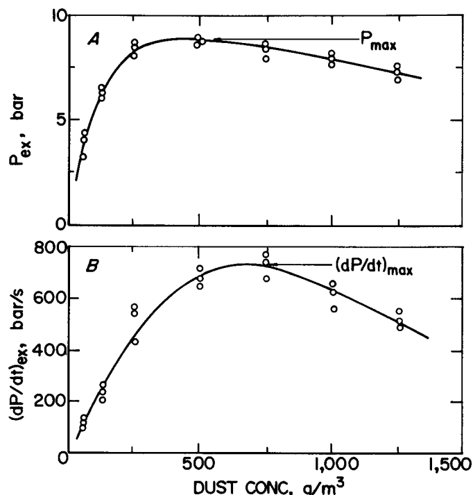
FIG. 2 P_{\text{max}} and (dP/dt)_{\text{max}} as a Function of Concentration for a Typical Dust in a 20-L Chamber
