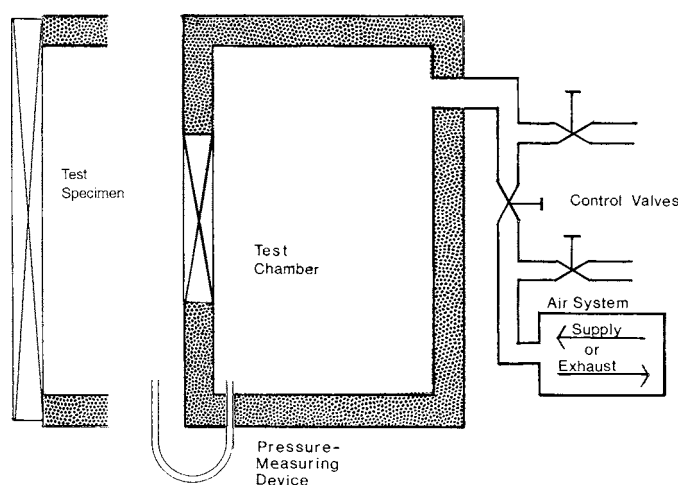
FIG. 1 General Arrangement of Testing Apparatus
