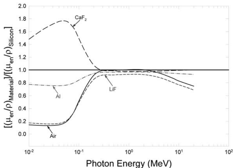
FIG. X4.1 Ratios of Mass Energy Absorption Coefficients of Various Materials Relative to That of Silicon
