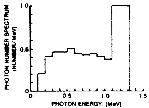
FIG. X1.6 Typical Spectra for Water Well Sources Under Various Conditions (4, 6)
