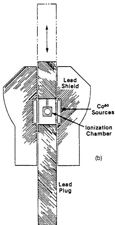
FIG. X1.7 Diagram of a Typical Shielded-Cavity Irradiator (5)
