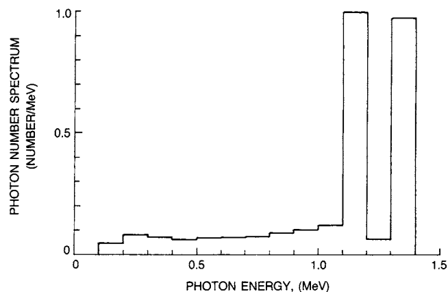
FIG. X1.2 Typical Spectra for Two Types of Teletherapy Sources a(2) and b(4)
