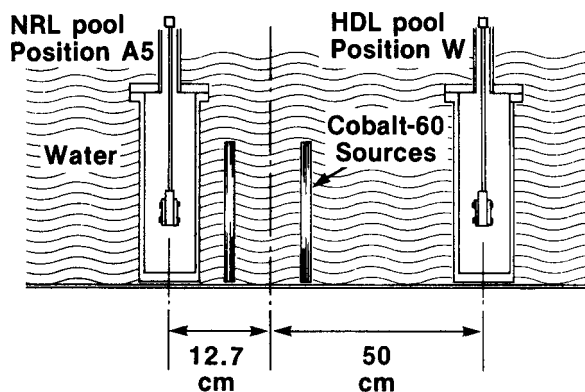
FIG. X1.5 Diagrams of Two Types of Water Well Sources (5)
