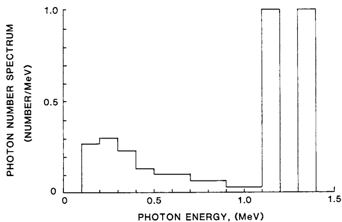
TELETHERAPY SOURCE
