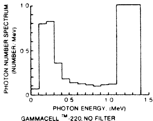
FIG. X1.8 Typical Spectrum for Shielded-Cavity Irradiator (4)
