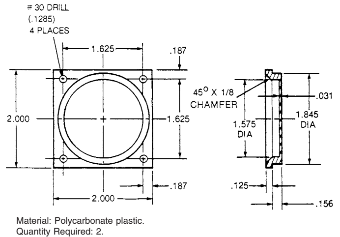
NOTE 1—1 in. = 25.4 mm. FIG. X2.5 Ionization Chamber Cover
