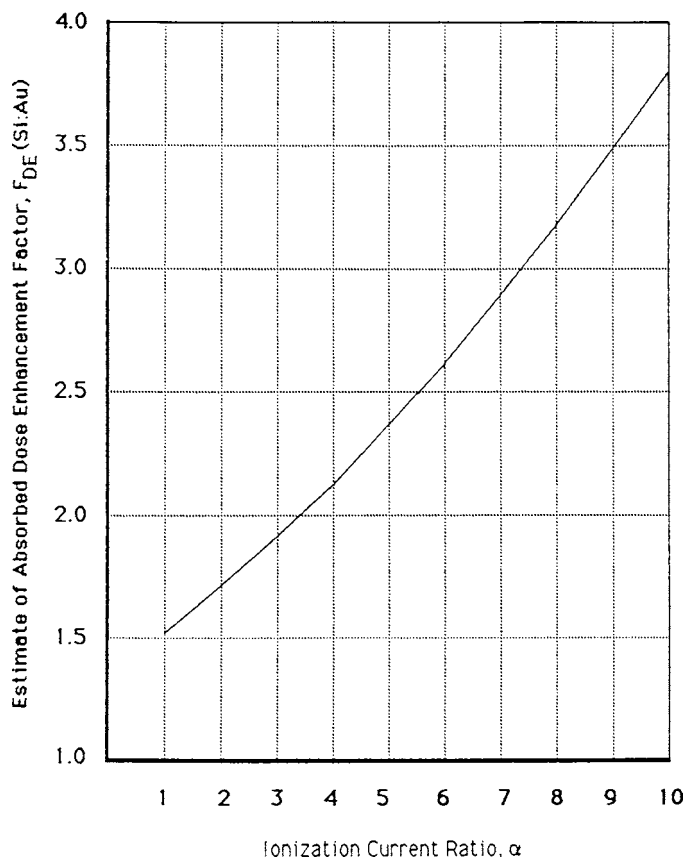
FIG. 2 Relationship for Estimating Absorbed Dose Enhancement Factor in Silicon at a Silicon-Gold Interface From the Ionization Current Ratio
