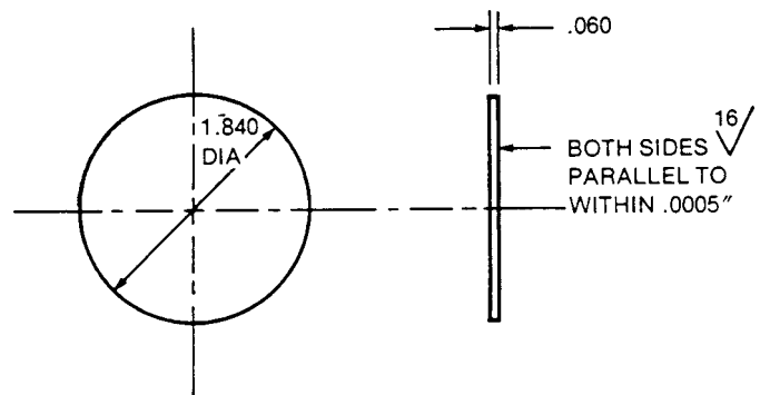
NOTE 1—1 in. = 25.4 mm. FIG. X2.5 Ionization Chamber Cover
