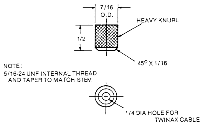
FIG. X2.7 Ionization Chamber Stem
