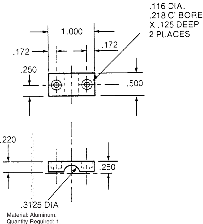
NOTE 1—1 in. = 25.4 mm. FIG. X2.4 Ionization Chamber Clamp
