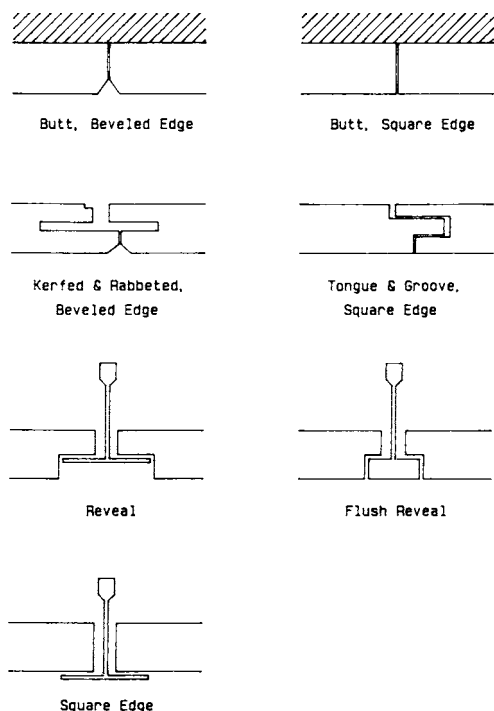
FIG. 1 Edge and Joint Details
