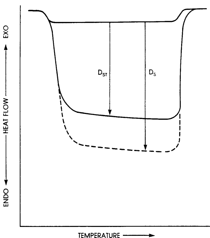
FIG. 1 Specific Heat Capacity Thermal Curves of Standard Sapphire, and Unknown Specimens
