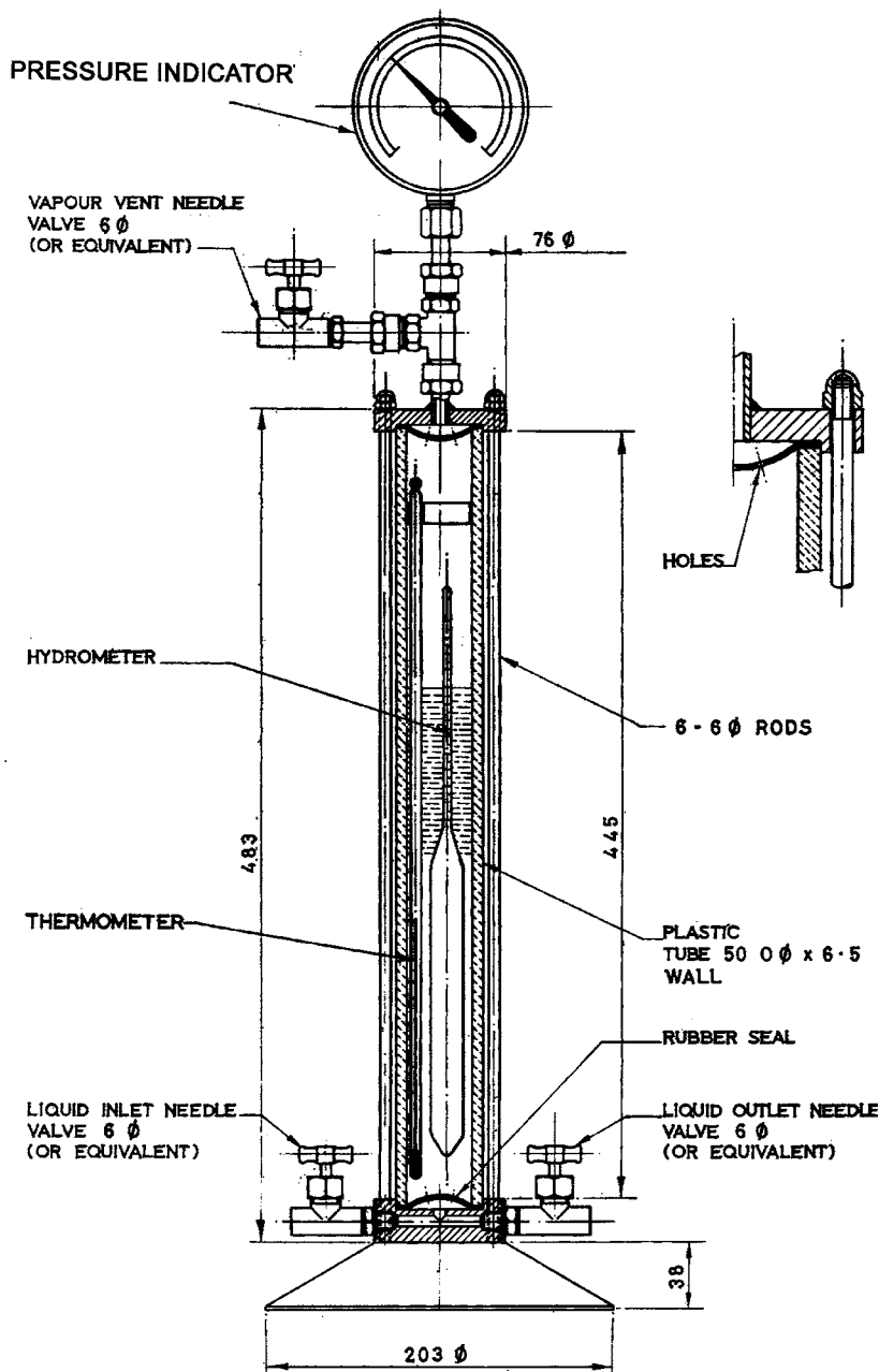
FIG. X1.2 Pressure Hydrometer Cylinder Comparator
