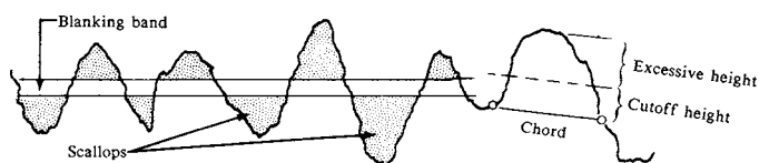
FIG. 1 Typical Profilograph
