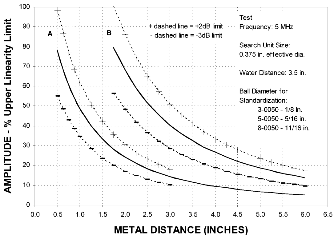
FIG. 6 Distance-Amplitude Response Curves (A and B) Showing the Interrelationship Between Ultrasonic Standard Reference Blocks of Various Lengths and Containing Flat-Bottom Holes
