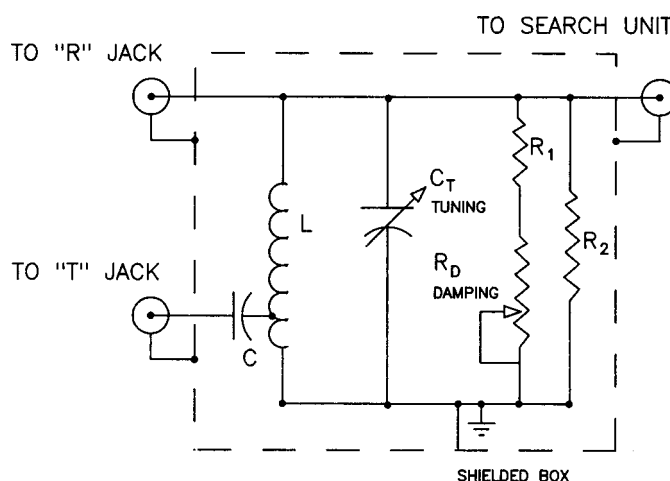
FIG. X1.1 Schematic Diagram for Tuning Network
