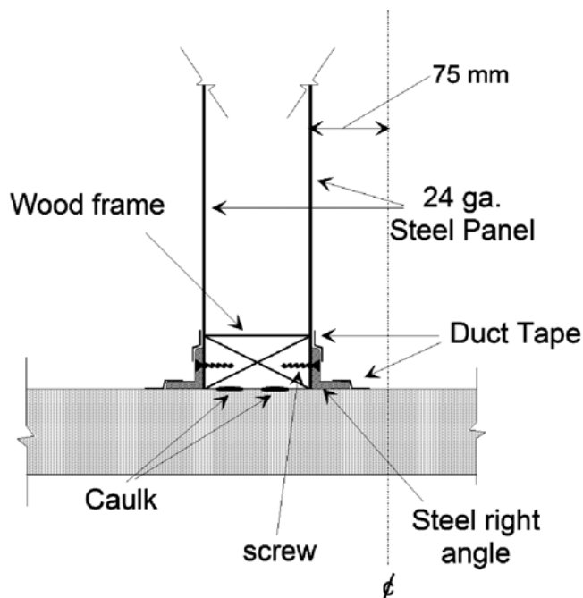
FIG. 5 Installation of Steel panels as double layer specimen on a single wood frame. The centerline symbol, c, represents the mid-plane of the test opening between two rooms.
