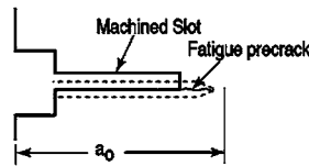
FIG. 8 Envelope of Fatigue Crack and Crack-Starter Notches
