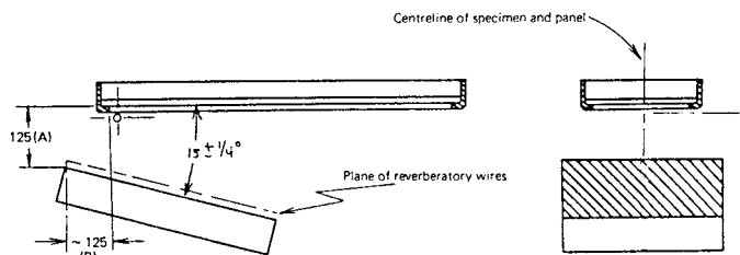
FIG. A1.1 Specimen and Panel Arrangement
