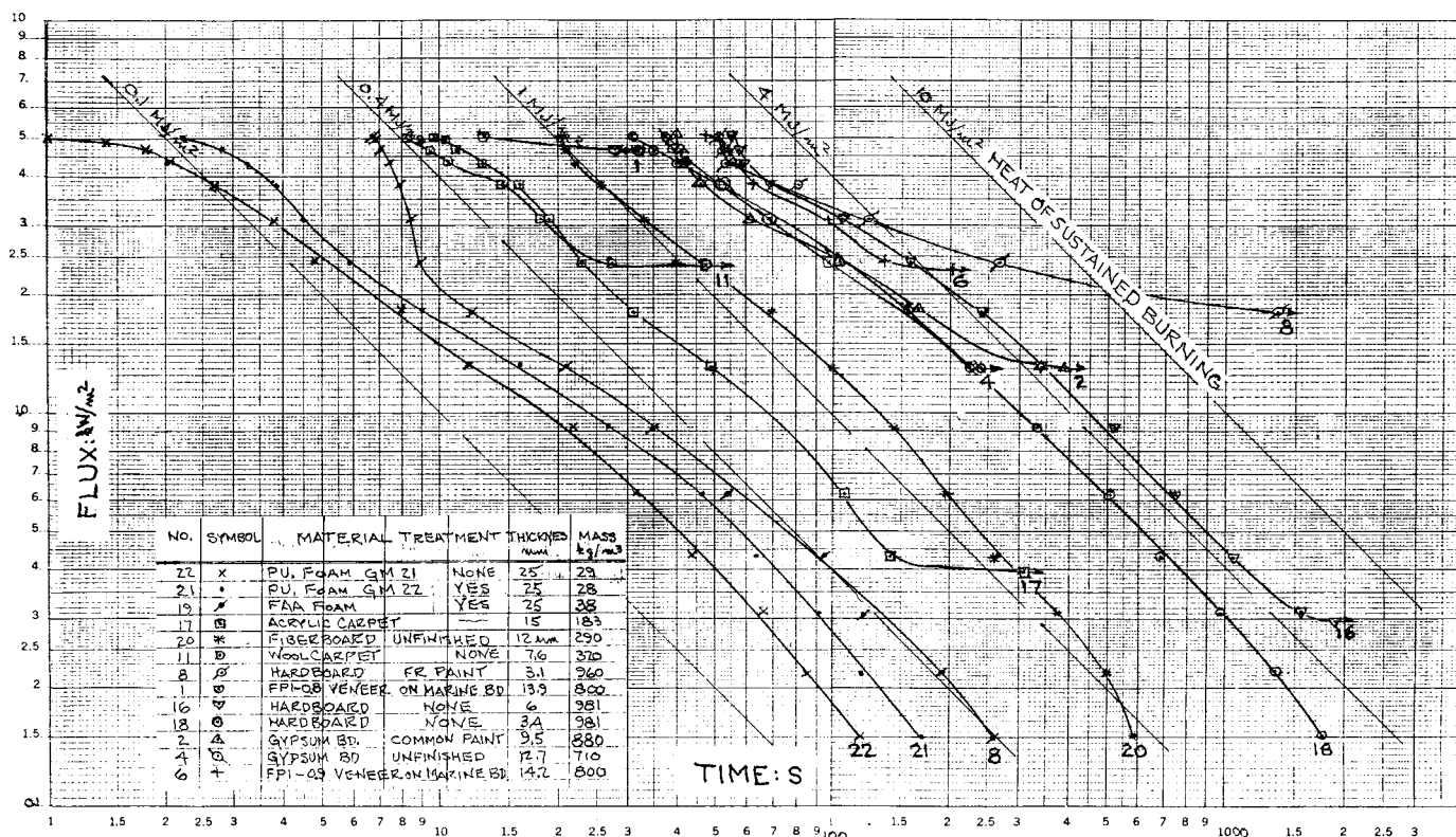
NOTE—A number of lines of constant heat of burning are included for reference. FIG. X1.3 Data From a Wide Range of Materials Plotted as Flux at Flame Front Versus Time
