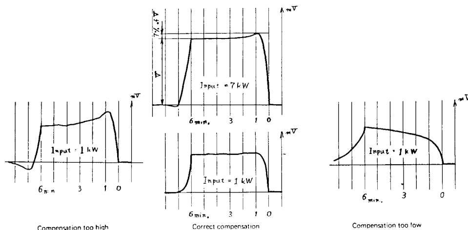
NOTE—The four curves shown illustrate changes in the indicated mV signal rise for three different levels of inverse feedback or compensation level. FIG. A1.4 Response-Behavior of Heat Release Signal to a Square Wave Thermal Pulse
