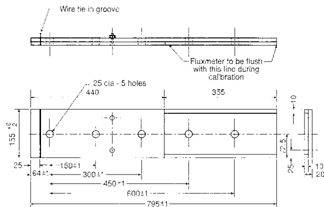
NOTE 1—All dimensions are in millimetres. FIG. 1 Dummy Specimen for Flux Gradient Calibration
