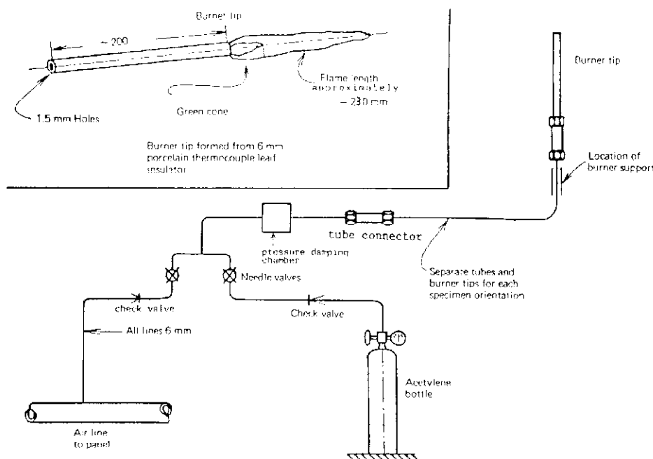
FIG. 8 Pilot Burner Details and Connections
