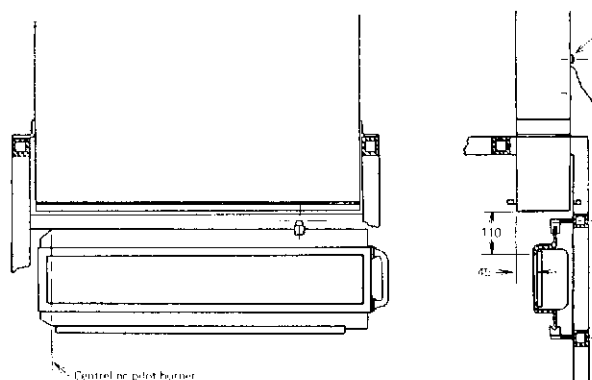
FIG. 7 Stack—Specimen Position Dimensions
