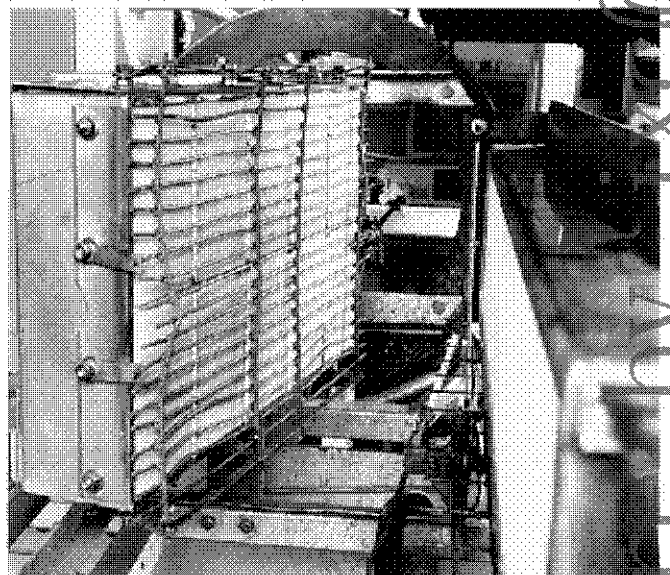
FIG. 4 Radiant Panel Facing Dummy Specimen
