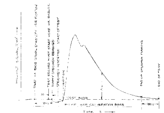
(a) Events Specified and Stack Millivolt Signal Curve Produced During Test
