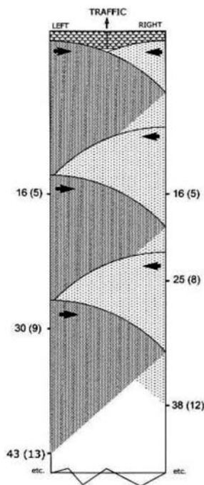
FIG. 1 Straightedge Positions
