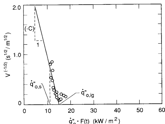
(a) Asphalt Shingle, \dot{q}''_e F(t) (kW/m 2 )
