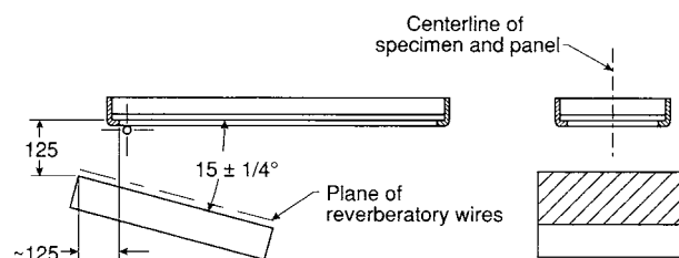
FIG. A1.2 Specimen-Panel Arrangement
