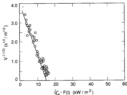
(b) Wool Carpet, \dot{q}''_e F(t) (kW/m 2 )
