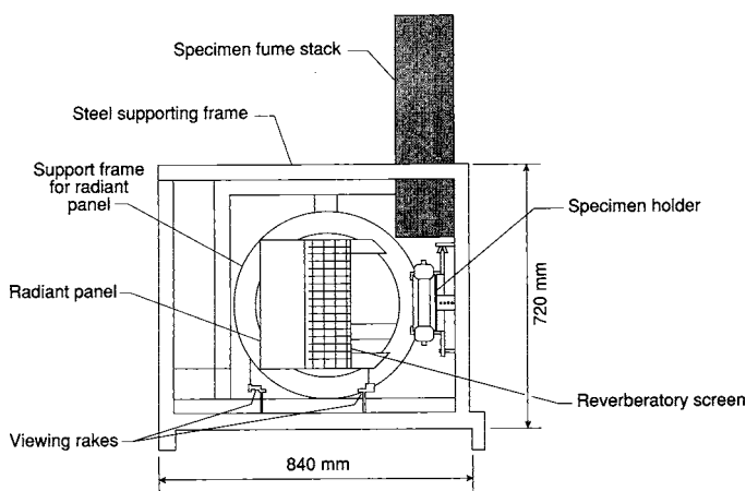
FIG. 6 Test Apparatus, Side View
