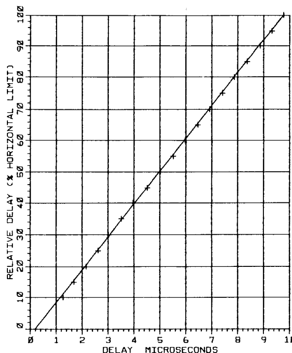
FIG. 9 Horizontal Linearity
