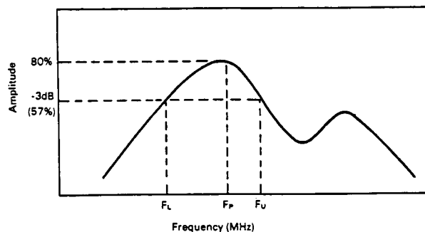
FIG. 8 Receiver Section Frequency Characteristics
