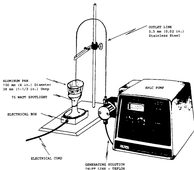
FIG. X2.1 Equipment Description
