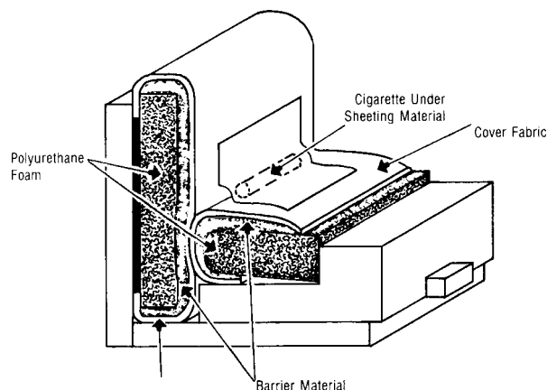
FIG. 9 Barrier Materials Test Method
