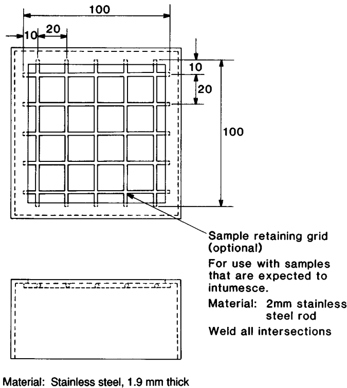
FIG. 8 Optional Wire Grid (For Horizontal or Vertical Orientation)
