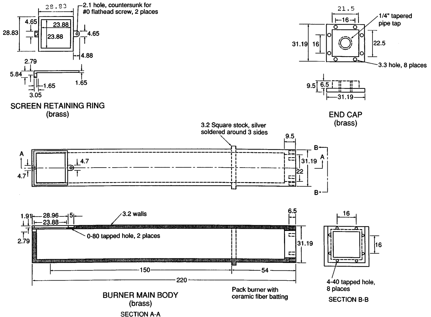
FIG. 11 Calibration Burner
