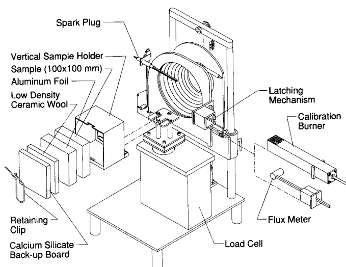
FIG. 4 Exploded View, Vertical Orientation
