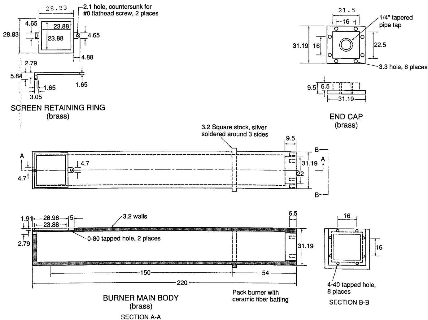
FIG. 11 Calibration Burner
