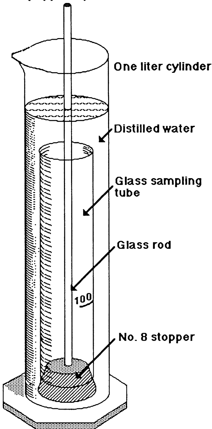
FIG. 5 Devices for Scraping, Mixing, and Subsampling Microcosms (11.1 and 11.2.1)
