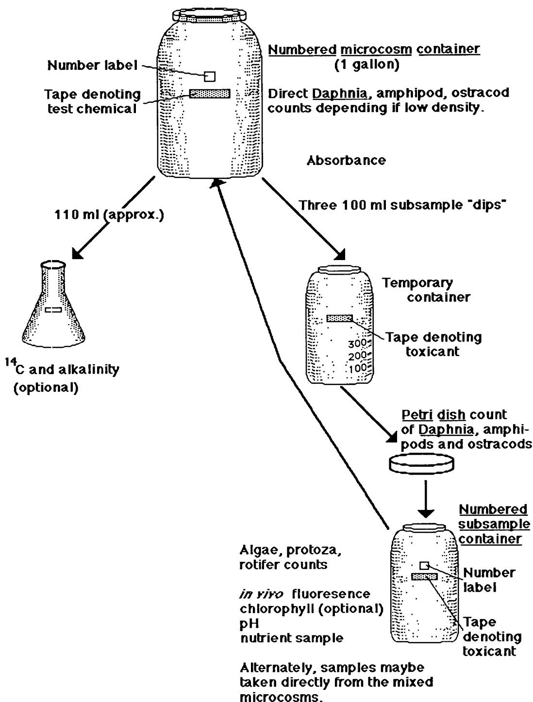
FIG. 6 Subsampling Progression for Counting Daphnia , Amphipods, and Ostracods (11.5.6.2(a))
