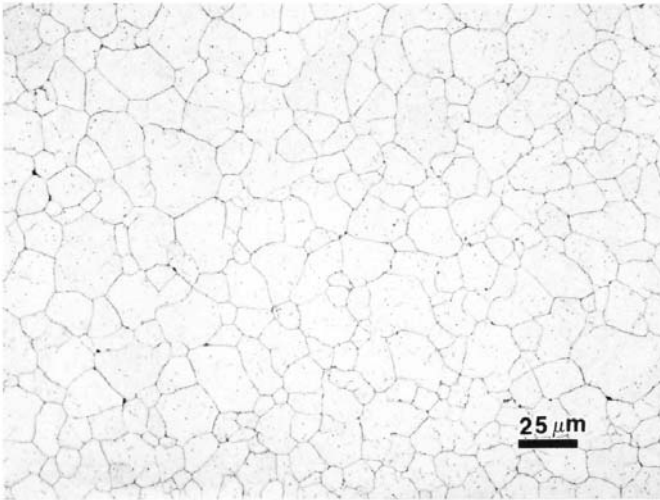
FIG. A2.6 Prior-austenite grain boundaries in this hot-worked tool steel specimen were decorated with cementite/pearlite by an isothermal hold at 1300°F (704°C) after austenitization (glyceregia etch). The boundaries are reasonably well developed and the specimen can be analyzed with a digitizing tablet but some editing would be required for automatic image analysis.
