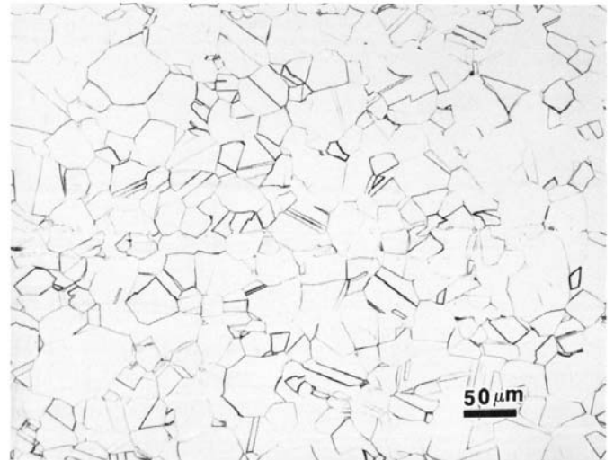
FIG. A2.11 Austenitic grain structure of AISI 316L stainless steel revealed using waterless Kalling's reagent. A substantial percentage of the grain boundaries are not visible and the annealing twins are revealed. The grain structure is too poorly revealed for successful image editing.
