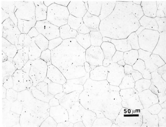
FIG. A2.7 Prior-austenite grain boundaries in a solution annealed 18Ni250 maraging steel revealed by electrolytic etching with aqueous 10 % \text{CrO}_3 (9 A/cm 2 , 5 min). There are a number of missing grain boundaries that must be added before measurement.
