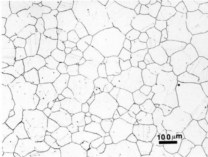
FIG. A2.9 Austenitic grain structure of solution annealed and double aged Waspaloy revealed using glyceresia. Some grain boundaries are missing. The faint annealing twins would interfere with automatic image analysis but not measurement with a digitizing tablet.
