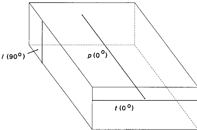
FIG. A1.2 Alternate Test Line Orientations Plate or Sheet Products
