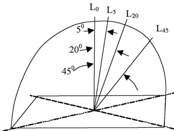
FIG. 1 Measurement Angles of Divergence and Dispersion of Light
