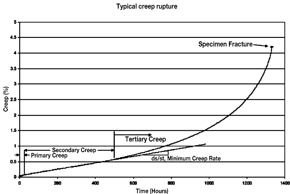
FIG. 3 Typical Creep Curve
