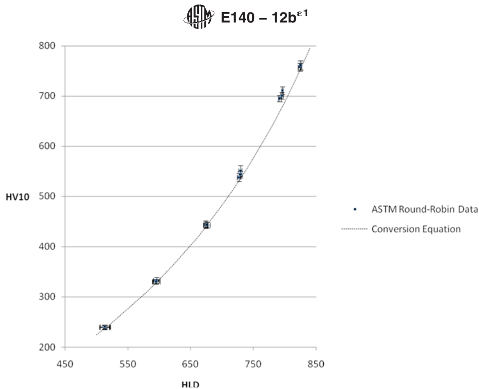
FIG. X2.3 Comparison of Mean Values of Subcommittee E28.06 Round-Robin Data to Conversion Eq A10.3 (Conversions from Leeb D hardness to Vickers hardness). The standard deviation of subcommittee E28.06 round-robin data is shown as error bars for each respective data point. R^2=0.9931 for the data shown in this figure.
