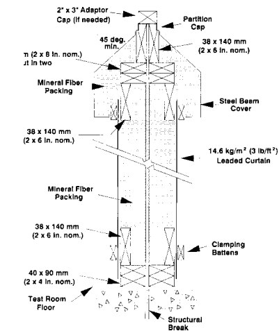
FIG. 2 Vertical Section Through a Partition Found to Satisfy the Requirements of 7.2
