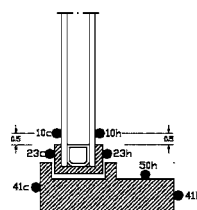
FIG. 9 Glazed Walls and Sloped Gllazing Temperature Sensor Placement
