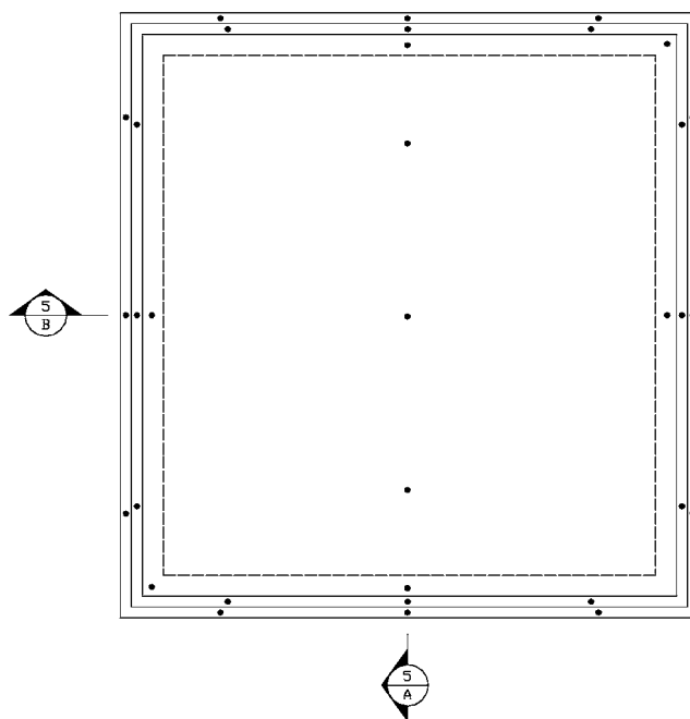
FIG. 7 Fixed Window Temperature Sensor Placement
