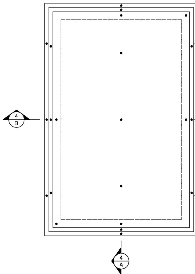
FIG. 5 Sidelite and Transoms Temperature Sensor Placement (Transoms - Rotate 90°)
