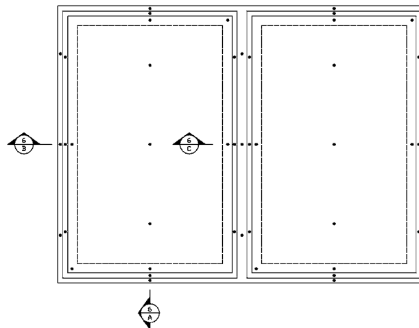
FIG. 9 Glazed Walls and Sloped Gllazing Temperature Sensor Placement
