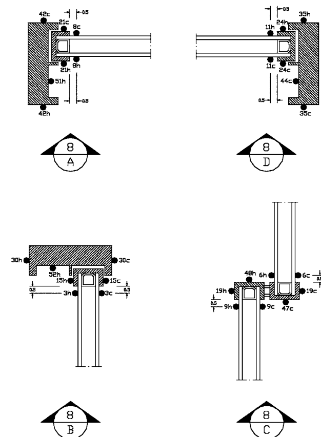
FIG. 14 Cross-sections of Vertical Slider Temperature Sensor Placement
