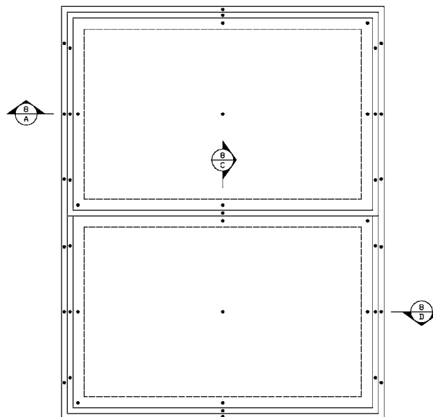
FIG. 13 Vertical Slider Temperature Sensor Placement
