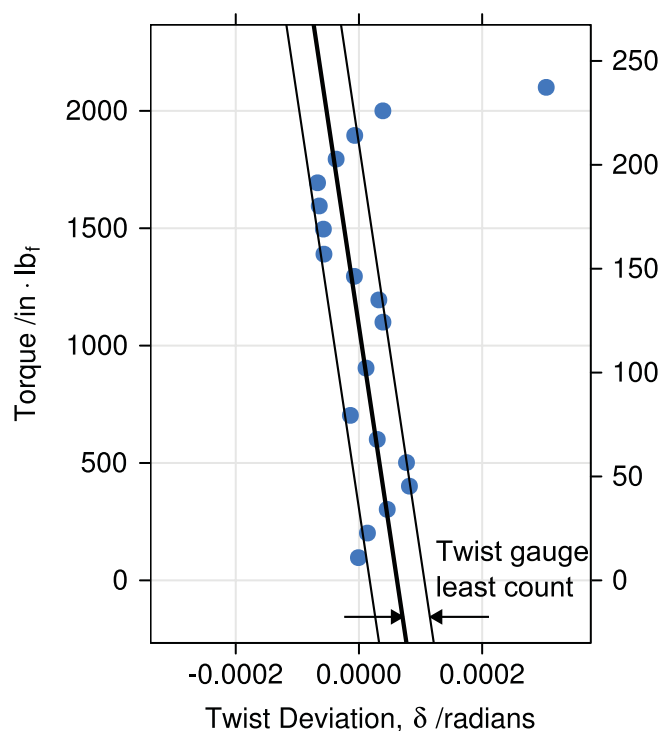
FIG. 2 Torque-Twist Deviation Graph
