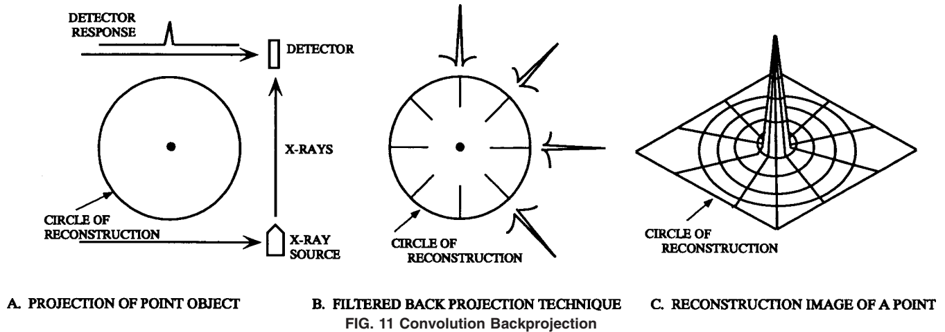
FIG. 11 Convolution Backprojection
