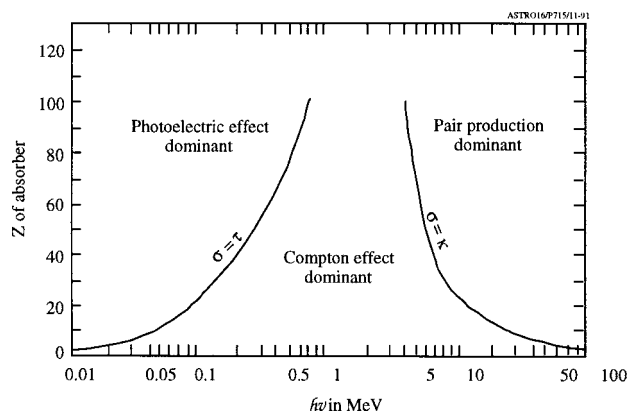
FIG. 7 Principal X-Ray Interactions
