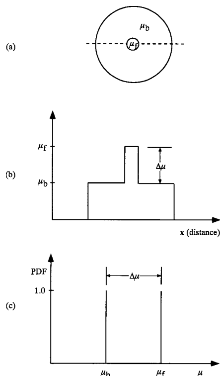
FIG. 13 (a) A Sketch Illustrating a CT Reconstruction of a Small Feature of Attenuation Coefficient \mu_f Embedded in the Center of a Background Material of Attenuation Coefficient \mu_b ; (b) A Plot of the CT Density Profile Through the Feature in (a); and (c) A Probability-Distribution Function (PDF) for the Attenuation Coefficients Found in (a)
